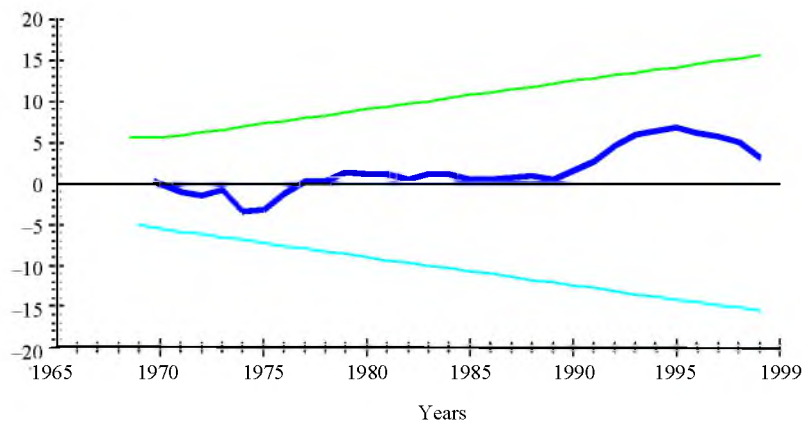
Fig. 1. Plot of Cumulative Sum of Recursive Residual and 5 Percent Significance Level Critical Bands.
